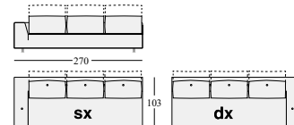
ABS270Tsx ABS270Tdx
