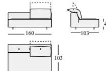
ABS160EC
