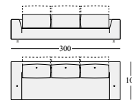
ABS300dv
